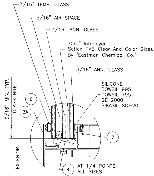
GLASS TYPE 'Ai' 15/16" OVERALL INSUL. LAM. GLASS
